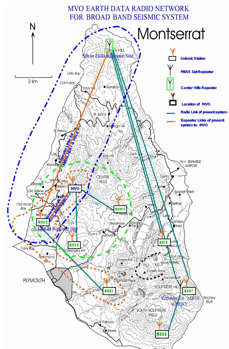
Figure 1: Map by Dave Williams indicating how the digital seismic telemetry would be realigned for transmitting data to MVO Flemings.
